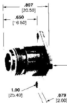
Part No. 135014-1
