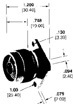
Part No. 135012-1
