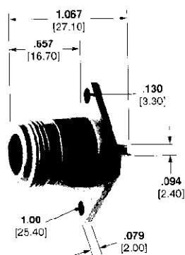
Part No. 134866-1
