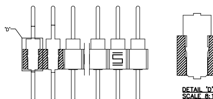
FIG "A" TD-1XX-X-X & TS-1XX-X-B SHOWN (SEE NOTE 6 & 10)
