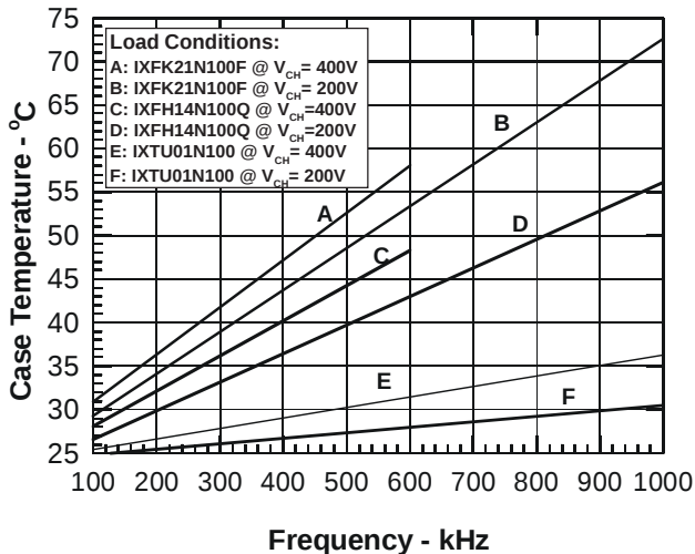
Fig. 27b. Case temperature rise vs. switching frequency for IX6R11S6
