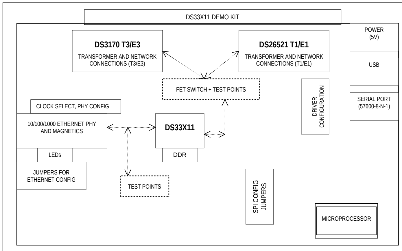
Figure 1-1. DS33X11 System Floorplan
