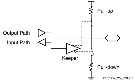
Figure 12: Keeper Circuit
