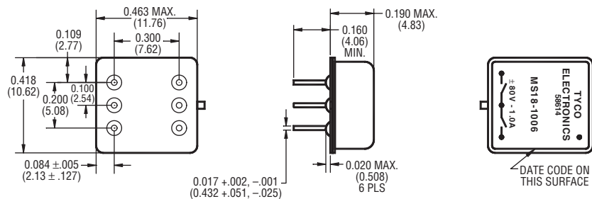
Figure 5 - Outline Dimensions
