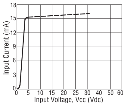
Figure 1 - Max. Input Current vs. Input Voltage
