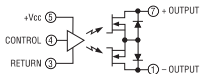
Figure 6 - Simplified Circuit
