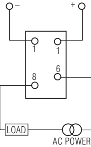
Terminal View
