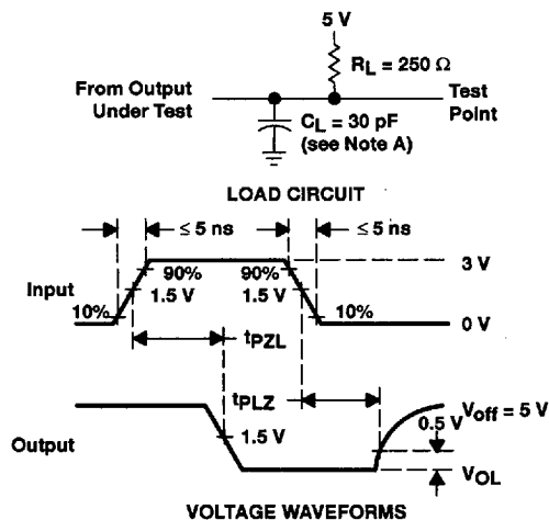
Figure 15. t_{pZL} and t_{PLZ} ( '118 and '119 receivers only)
