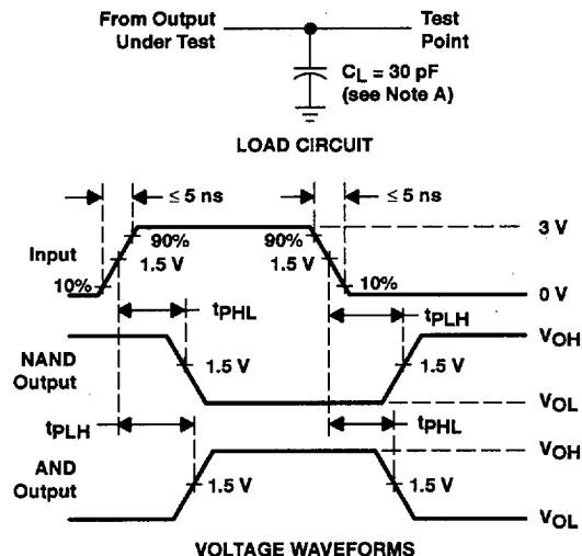
Figure 13. t_{PLH} and t_{PHL} (drivers only)
