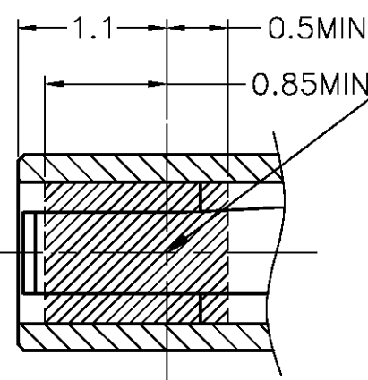
SECT. D-D (SCALE 20:1)
