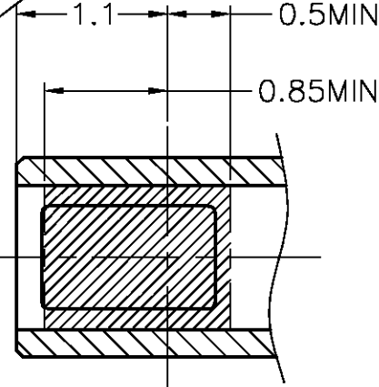
SECT. E-E (SCALE 20:1)
