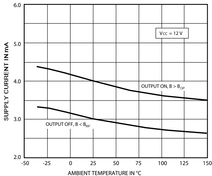
SUPPLY CURRENT
