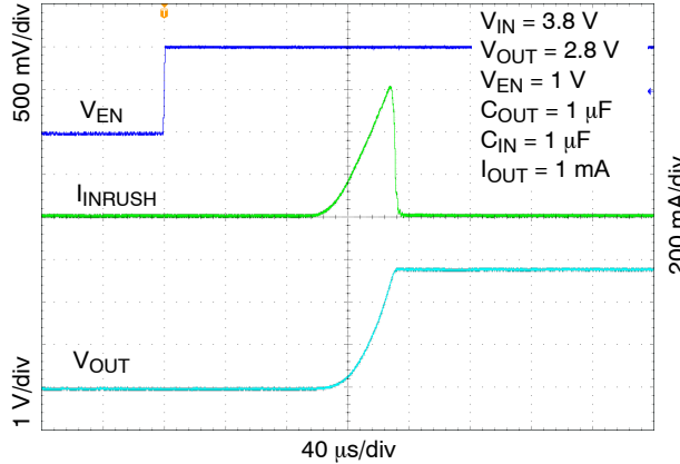
Figure 28. Enable Turn-on Response, C OUT = 4.7 \mu F, I OUT = 1 mA
