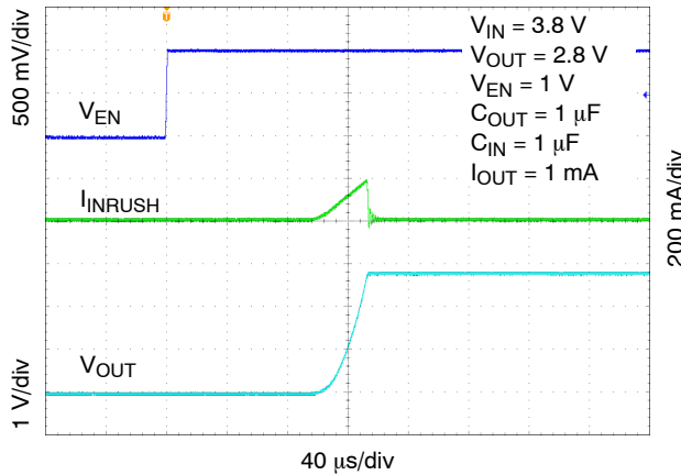
Figure 26. Enable Turn-on Response, C OUT = 1 \mu F, I OUT = 1 mA
