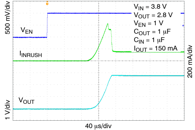
Figure 29. Enable Turn-on Response, C OUT = 4.7 \mu F, I OUT = 150 mA
