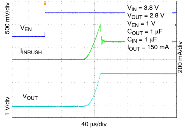
Figure 27. Enable Turn-on Response, C OUT = 1 \mu F, I OUT = 150 mA
