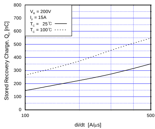
Fig 20. Stored Charge
