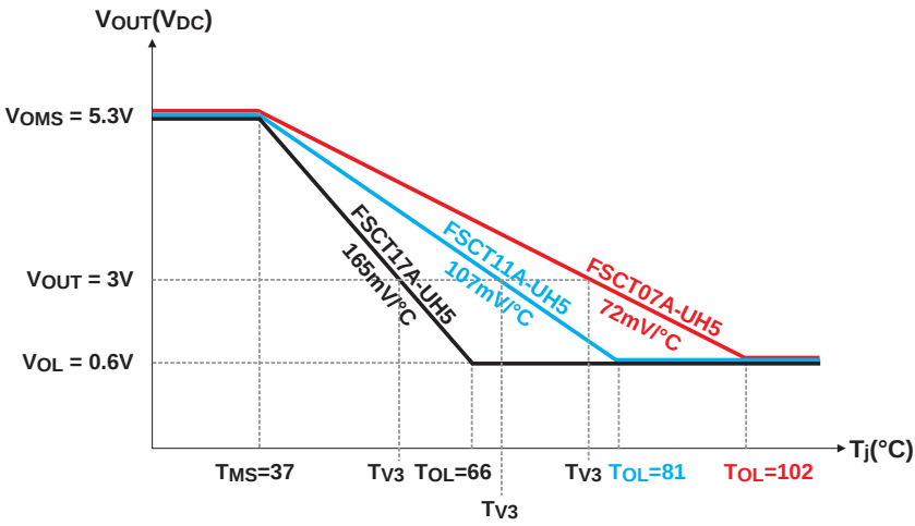
Fig. 3: Temperature slopes.
