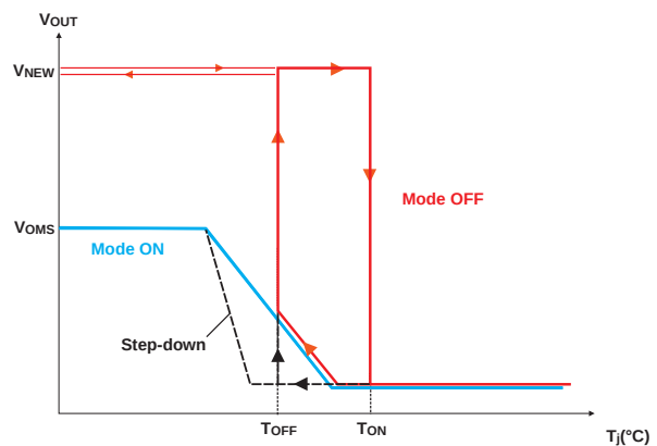
Fig. 12: Modified characteristics.
