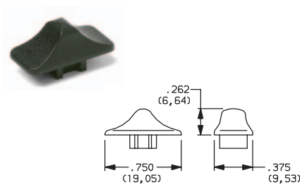
Cap Compatible with 01-05 actuators
