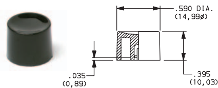
Cap Compatible with 13-19 actuators
