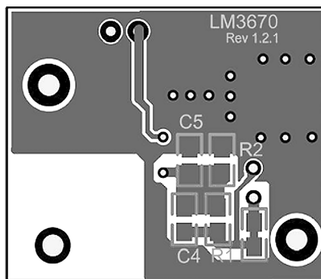
Figure 5. Bottom Layer
