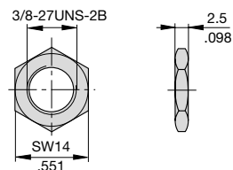
Hex nut 3/8" nickel-plated brass Y 300 192 01
