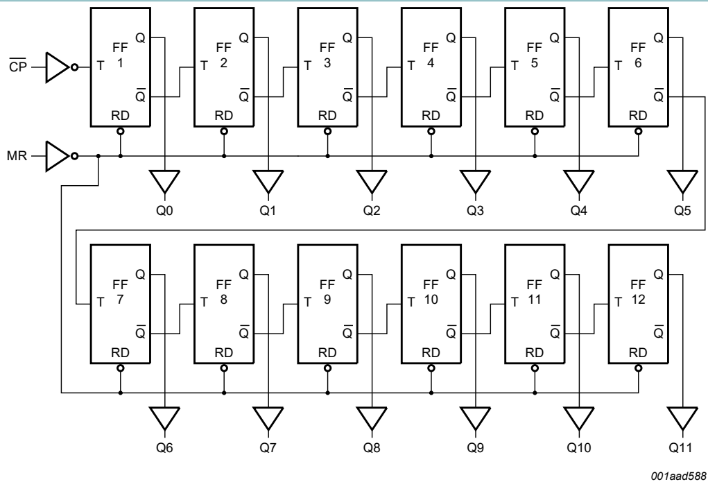
Fig. 4. Logic diagram
