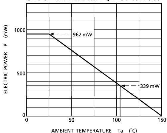
THE THERMAL RESISTANCE CHARACTER- ISTIC OF THE PACKAGE : QFP48-P-1014-0.80
