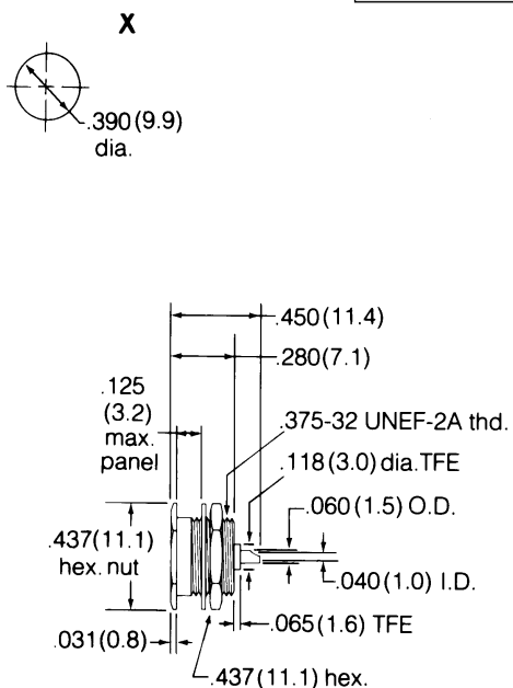
SMB Recessed Bulkhead Jack Receptacle Front Mount/Male Contact/Solder Cup Terminal 903-407J-51R Gold Plated
