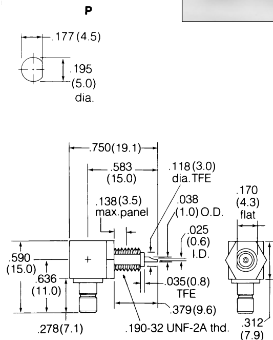
SMB Angle Bulkhead Jack Receptacle Front Mount/Male Contact/Solder Cup Terminal 903-416J-51R ▲□ Gold Plated
