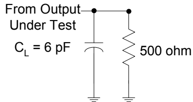
Figure 6. Load Circuit [8, 9, 10]
