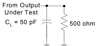
Figure 2. Load Circuit [4, 5, 6]
