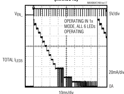
SINGLE-WIRE PULSE DIMMING (MAX8648)
