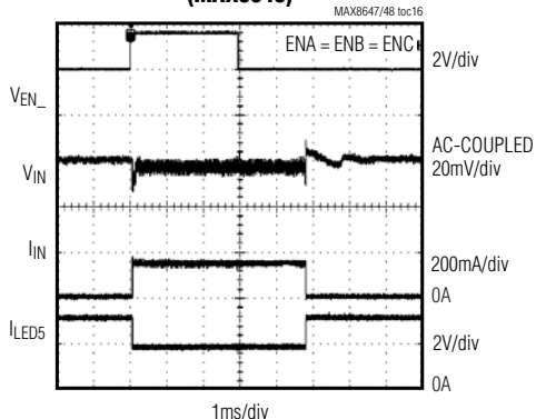
STARTUP AND SHUTDOWN (MAX8648)
