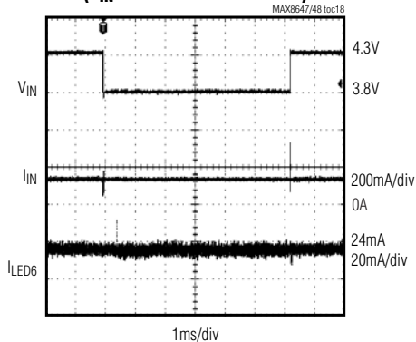
LINE-TRANSIENT RESPONSE ( V_{IN} = 4.3V TO 3.8V TO 4.3V )
