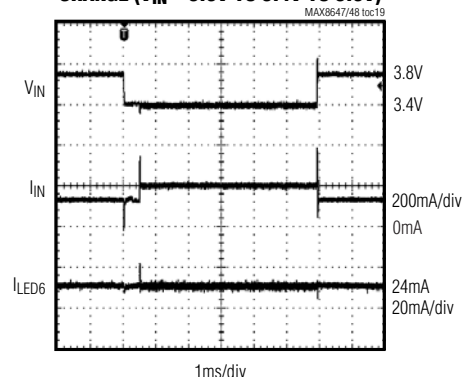
LINE-TRANSIENT RESPONSE WITH MODE CHANGE ( V_{IN} = 3.8V TO 3.4V TO 3.8V )
