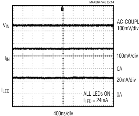
1x MODE OPERATING WAVEFORMS ( V_{IN} = 4V )
