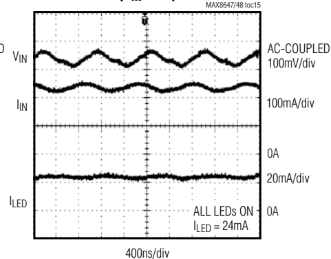
1.5x MODE OPERATING WAVEFORMS ( V_{IN} = 3V )
