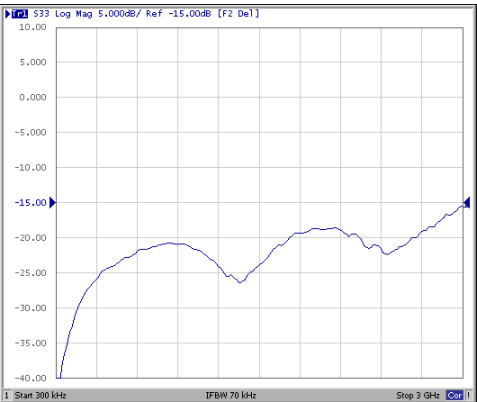
VJHD75TZ TYPICAL RETURN LOSS
