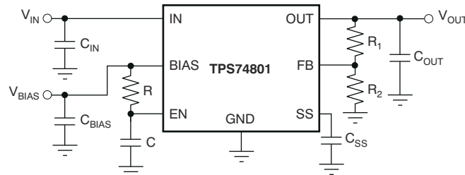
Figure 6-3. Soft-Start Delay Using an RC Circuit to Enable the Device
