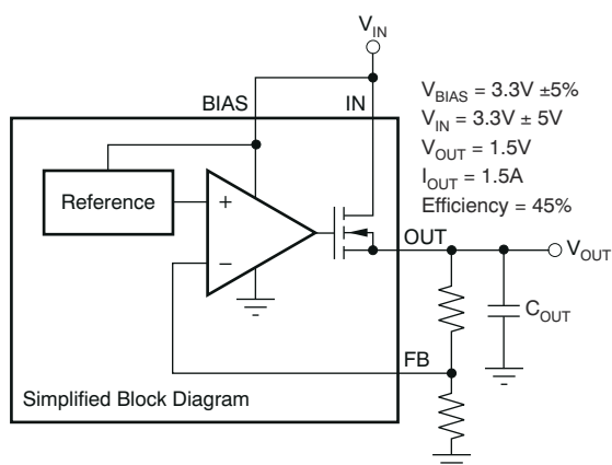
Figure 7-8. Typical Application of the TPS748 Without an Auxiliary Bias Rail
