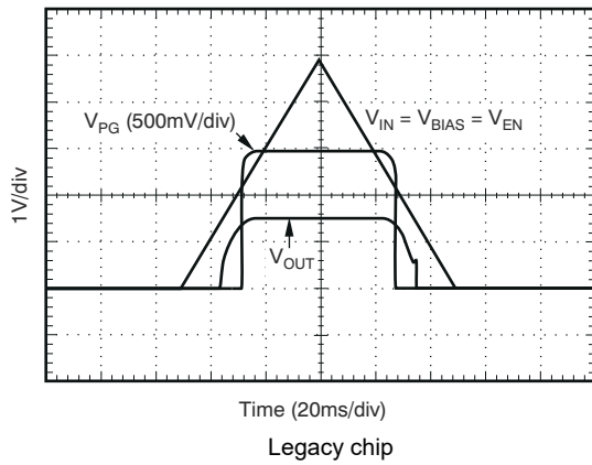
Figure 5-41. Power-Up, Power-Down
