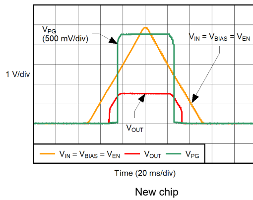
Figure 5-42. Power-Up, Power-Down
