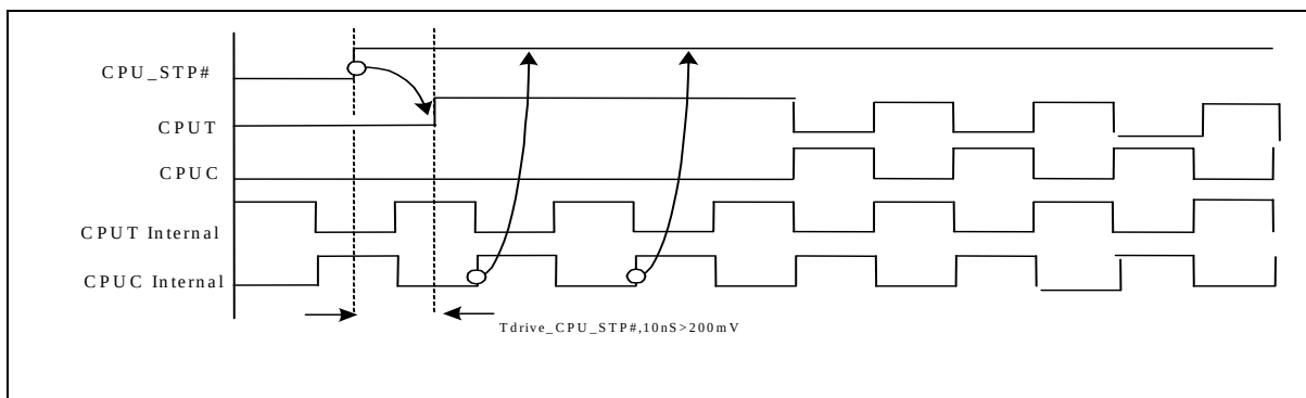
Figure 6. CPU_STP# De-Assertion
