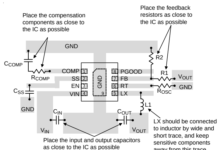
(b) For WDFN-8L 3x3 package
