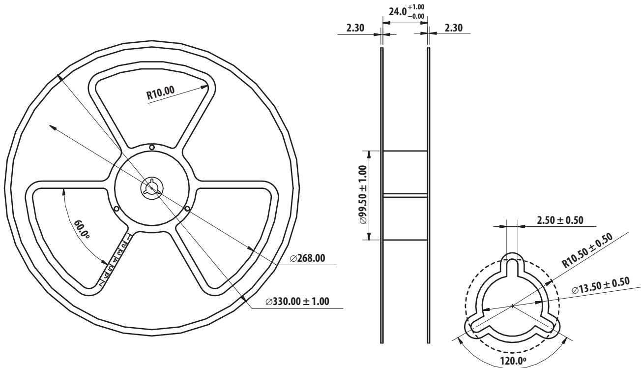
Figure 19. Reel dimensions.
