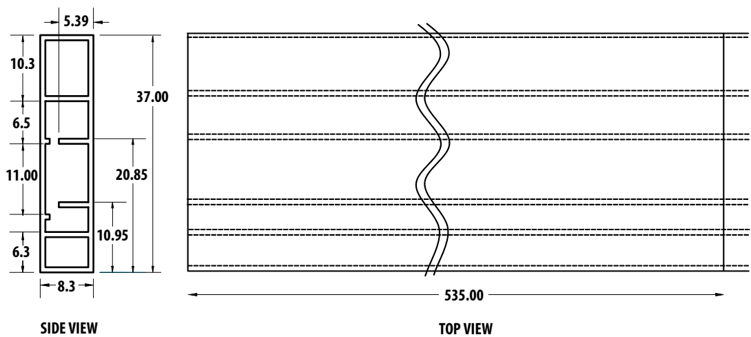
Figure 16. Tube dimensions.
