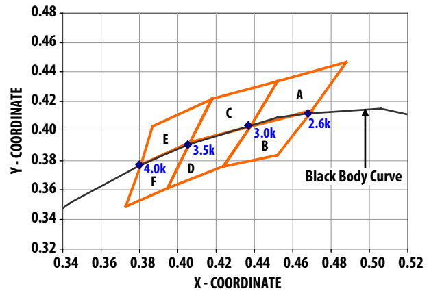
Figure 15. Color bins (Warm White).
