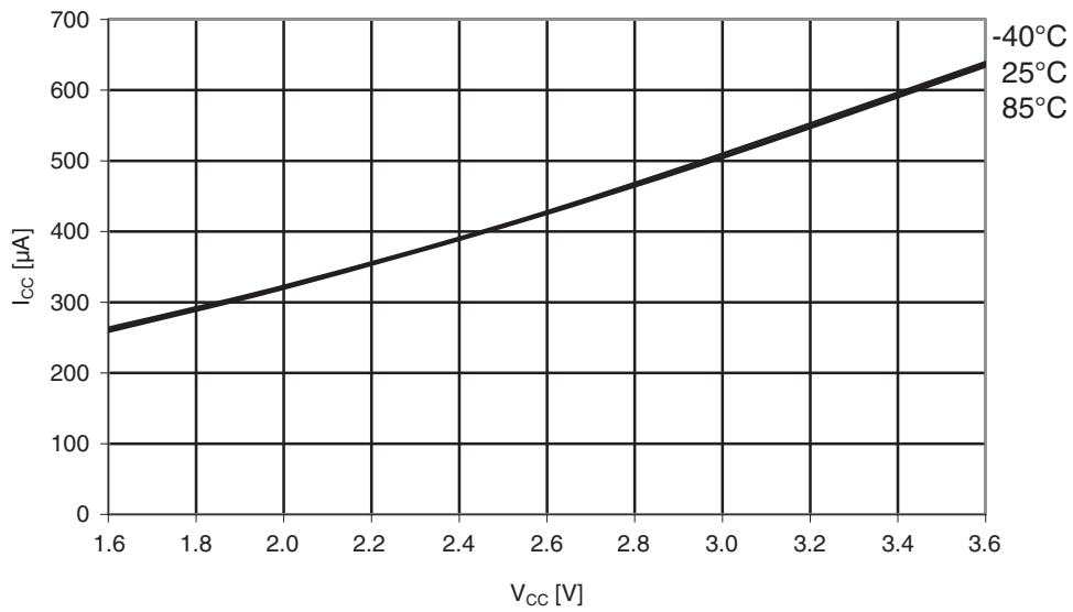
Figure 33-54. Idle supply current vs. V_{CC} . f_{SYS} = 2.0MHz internal RC.
