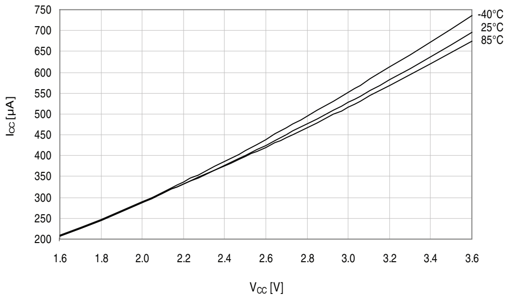
Figure 33-222. Active mode supply current vs. V_{CC} . f_{SYS} = 1MHz external clock.
