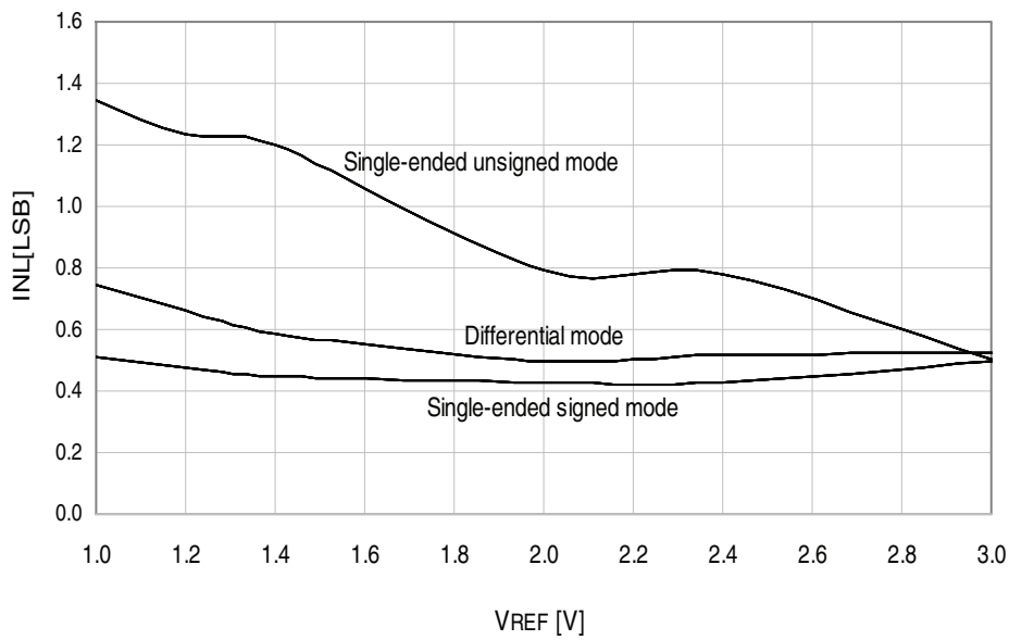
Figure 33-114. INL error vs. external V_{REF} . T = 25^\circ\text{C} , V_{CC} = 3.6\text{V} , external reference.
