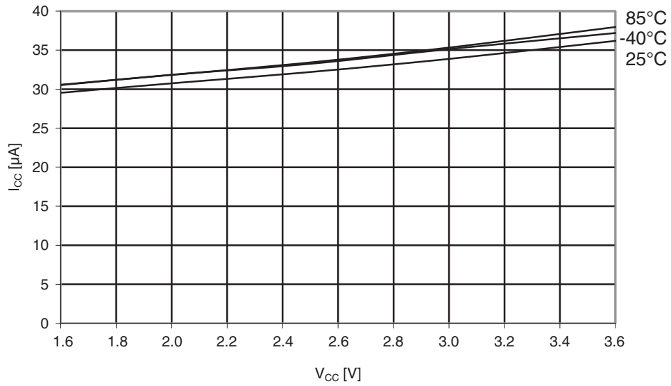
Figure 33-53. Idle supply current vs. V_{CC} . f_{SYS} = 32.768kHz internal RC.
