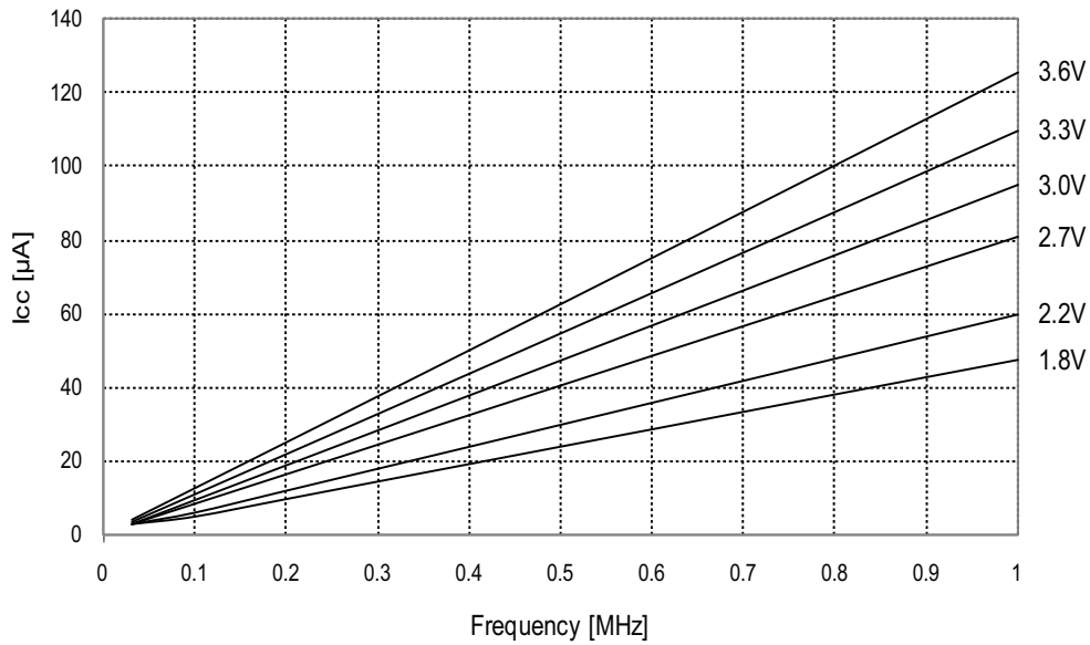
Figure 33-92. Idle supply current vs. frequency. f_{SYS} = 0 - 1.0MHz , T = 25°C .
