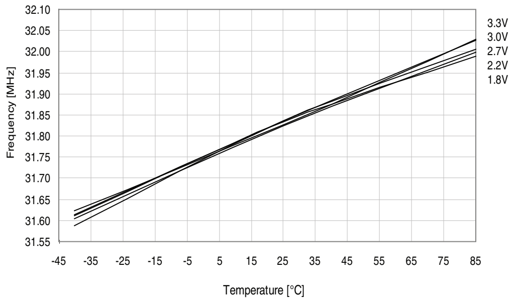
Figure 33-211. 32MHz internal oscillator frequency vs. temperature. DFLL enabled, from the 32.768kHz internal oscillator.
