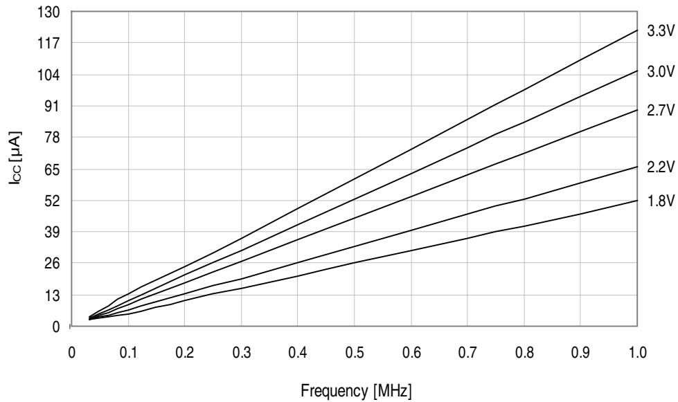
Figure 33-226. Idle mode supply current vs. frequency. f_{SYS} = 0 - 1\text{MHz} external clock, T = 25^\circ\text{C} .
