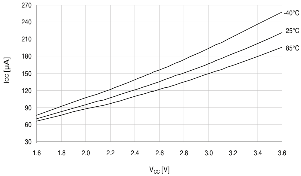
Figure 33-221. Active mode supply current vs. V_{CC} . f_{SYS} = 32.768kHz internal oscillator.
