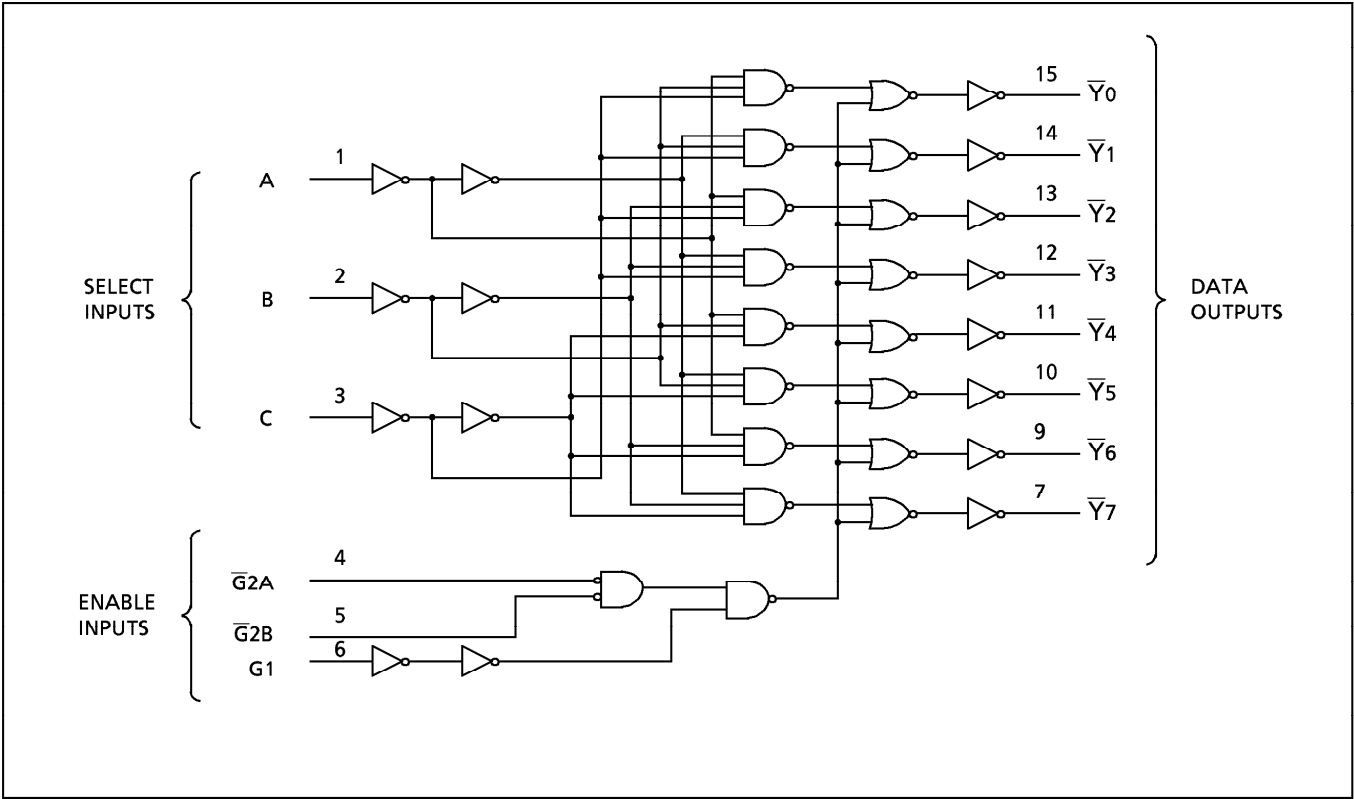
LOGIC DIAGRAM
