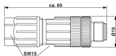
Dimensioned drawing
