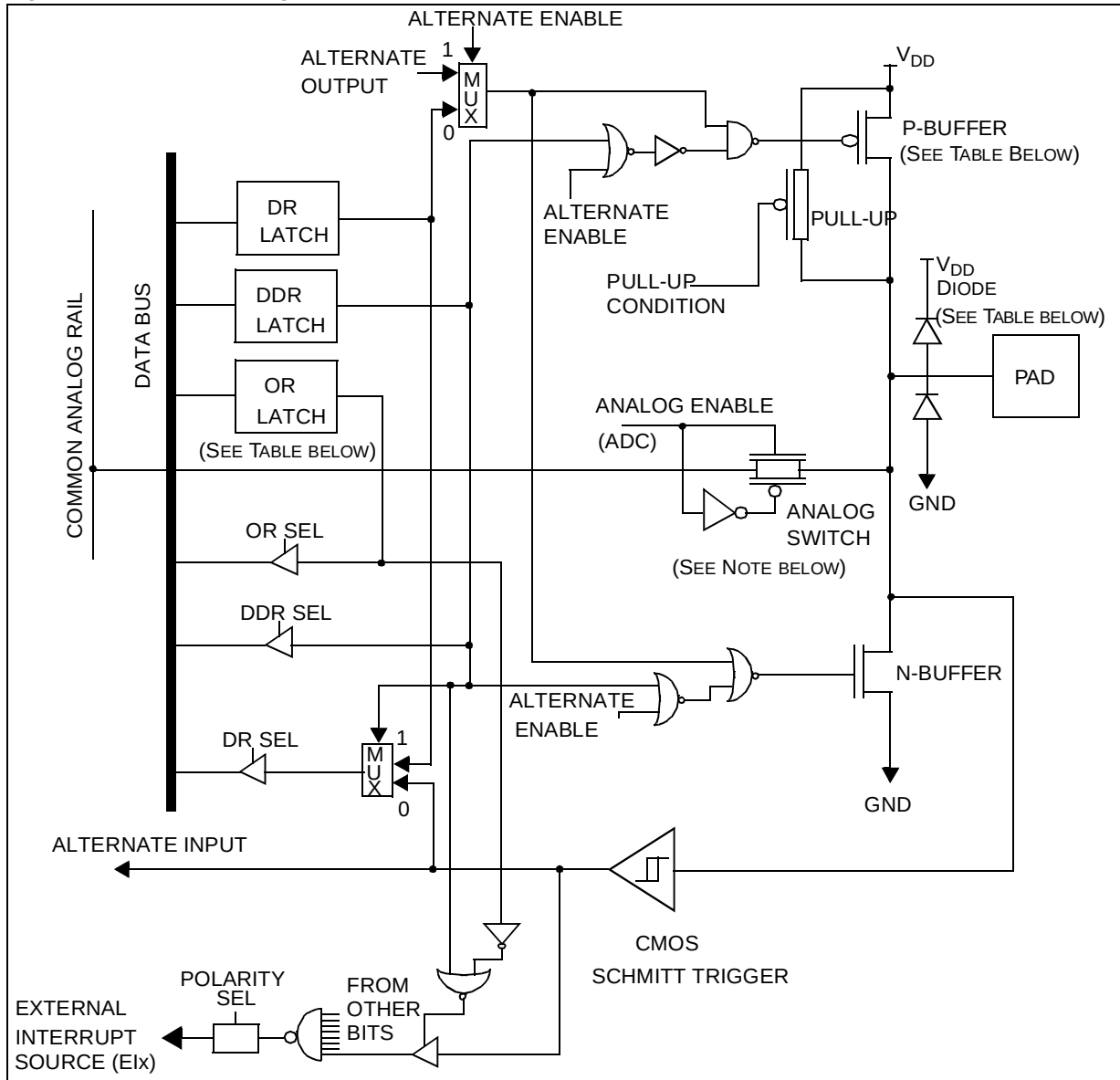
Figure 21. I/O Block Diagram
