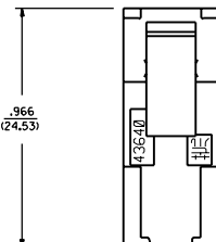
MATED MICRO-FIT CONNECTOR
