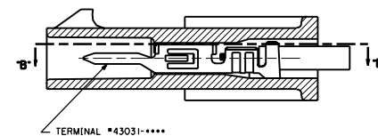
SECTION "D"-D" WITH TERMINAL (SCALE: 8X)
