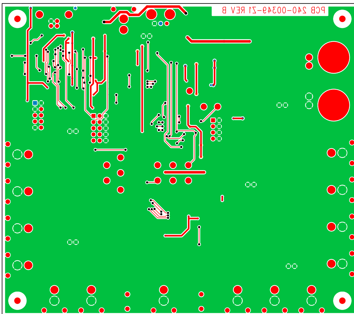
Figure 11. Bottom Layer
