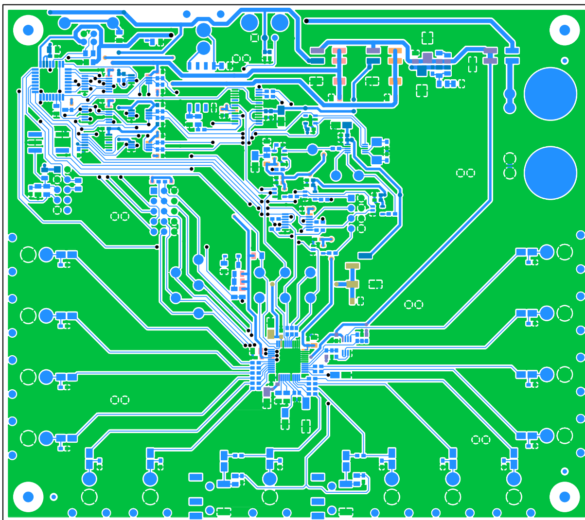
Figure 10. Top Layer
