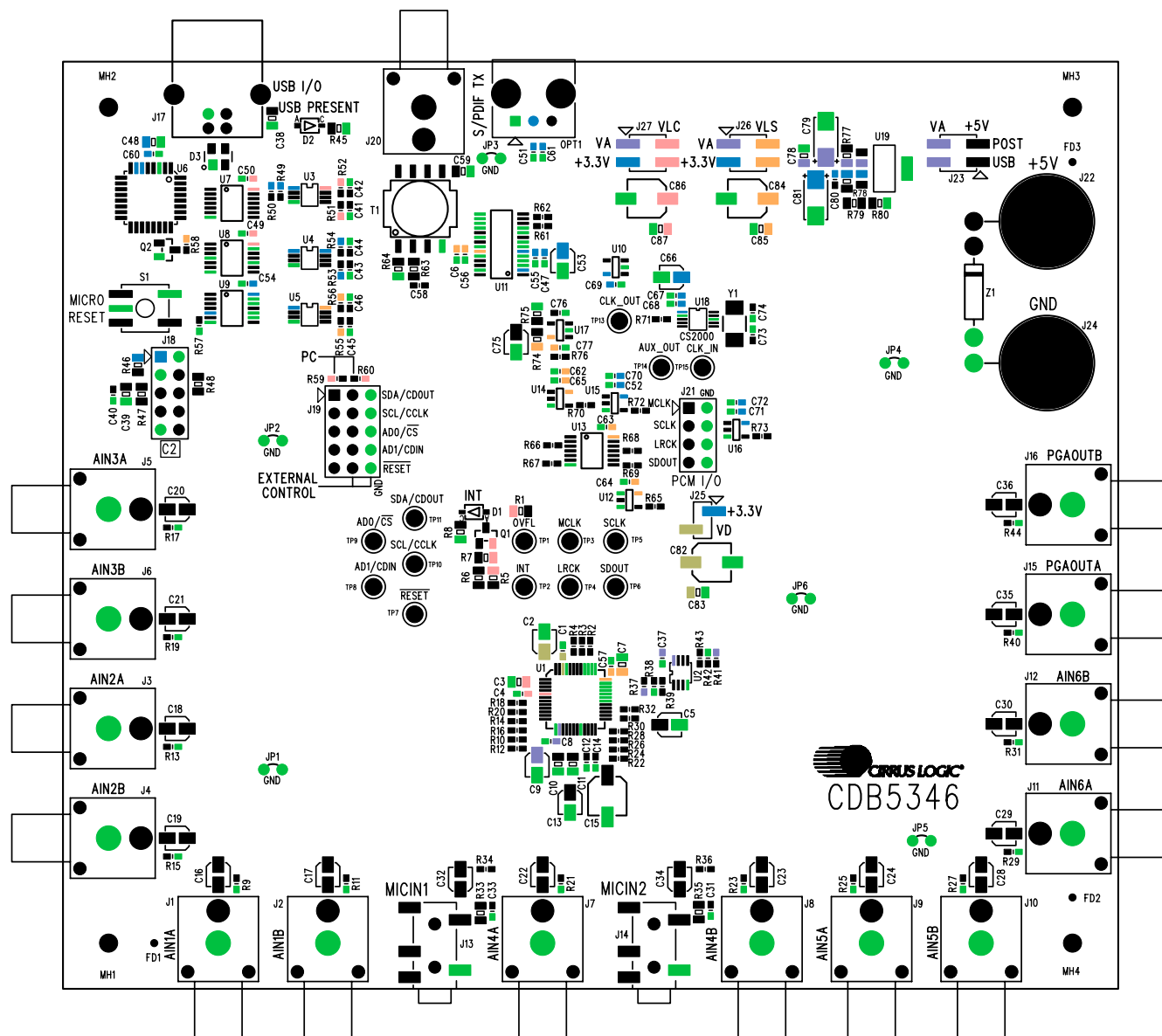
Figure 9. Component Map
