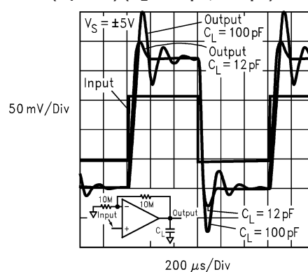
Small Signal Step Response ( A_V = +2 ) ( C_L = 12\text{ pF} , 100\text{ pF} )
