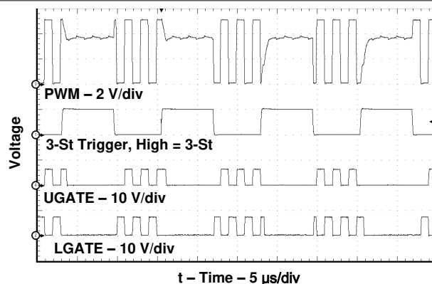
Figure 5-19. Normal and 3-State Operation Enter/Exit Conditions
