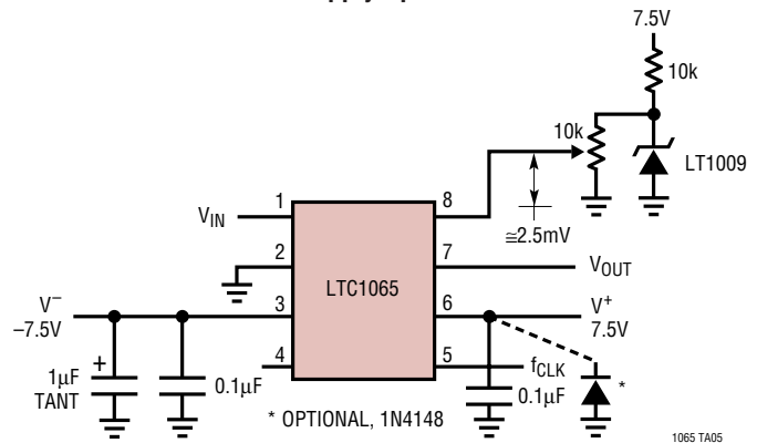
Adjusting V_{OS(OUT)} for \pm 7.5 Supply Operation
