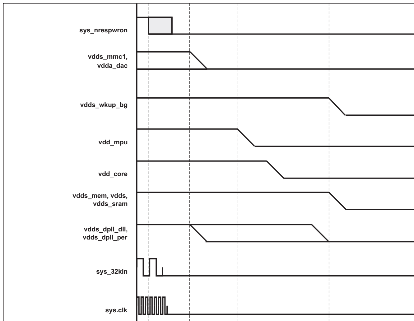
Figure 3-4. Power-down Sequence
