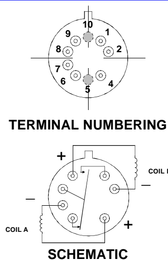
TERMINAL LOCATION, PIN NUMBERING AND SCHEMATIC ARE VIEWED FROM THE TERMINALS
