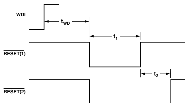
Figure 8. Watchdog \overline{RESET} Timing
