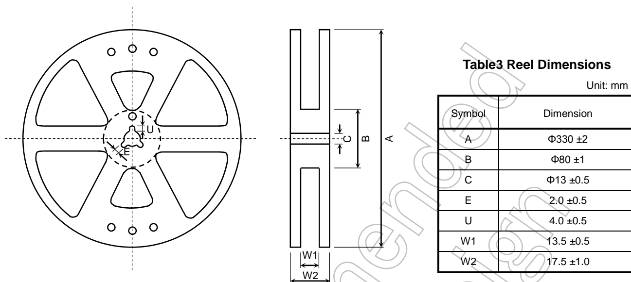
Figure 4 Reel Form
