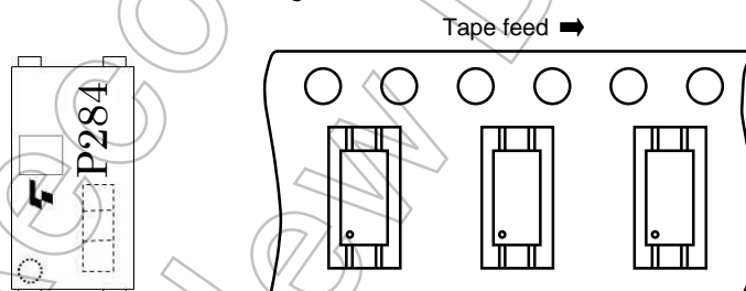
Figure 2 Device Orientation
