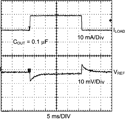
Load Transient Response I_{LOAD} = 0 \text{ to } 10\text{mA}
