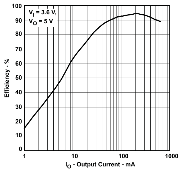
Figure 5. Voltage-Mode Efficiency
