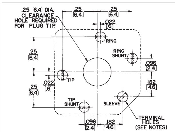
PARTIAL VIEW SHOWING SPRING LOCK TERMINALS Tip, ring and sleeve terminals are spring lock type.
