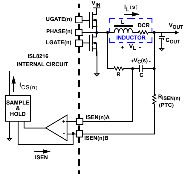
FIGURE 20. DCR SENSING CONFIGURATION
