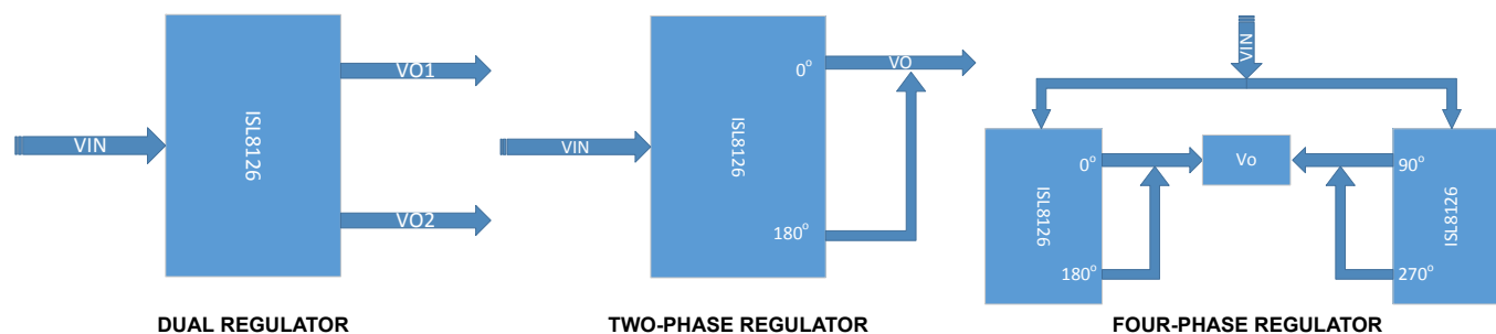
FIGURE 1. TYPICAL APPLICATION DIAGRAM
