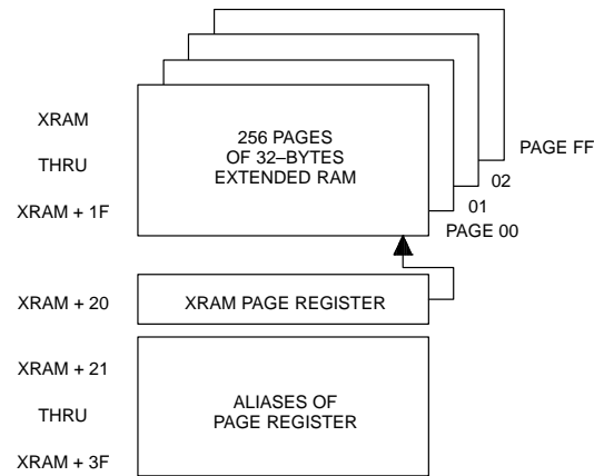
EXTENDED RAM ADDRESS MAP Figure 3
