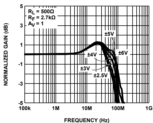
FIGURE 3. FREQUENCY RESPONSE FOR VARIOUS \pm V_S
