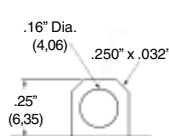
S 3 Solder Eye, extra large & quick connect
