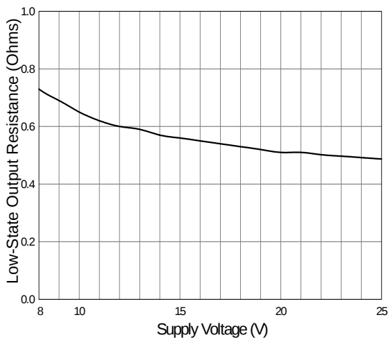
Low-State Output Resistance vs. Supply Voltage
