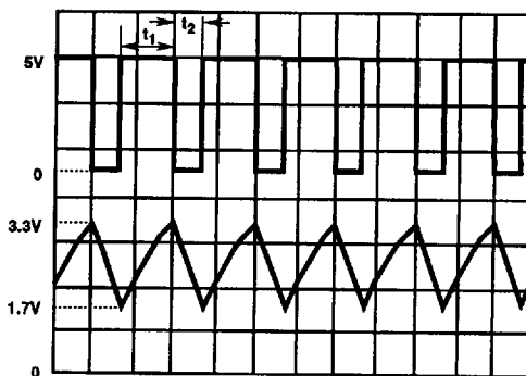
FIGURE 14. TYPICAL WAVEFORMS FOR REPEAT CYCLE TIMER
