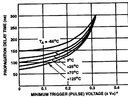
FIGURE 9. PROPAGATION DELAY TIME vs TRIGGER VOLTAGE
