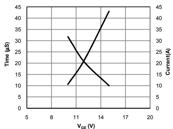
Fig 6: V_{GE} vs. Short Circuit Time ( V_{CE} = 400\text{V} , T_j = 25^\circ\text{C} )
