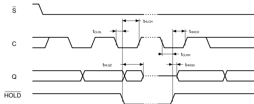
Figure 20. Hold timing
