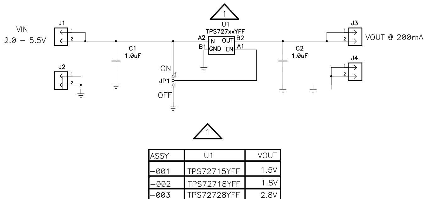
Figure 5. TPS727xxYFFEVM-407 Schematic
